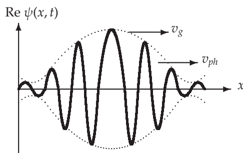
Figure 1.16: The function \text{Re } \psi(x, t) of the wave packet (1.123), represented here by the solid curve contained in the dashed-curve envelope, propagates with the group velocity v_g along the x axis; the individual waves (not drawn here), which add up to make the solid curve, move with different phase velocities v_{ph} .
