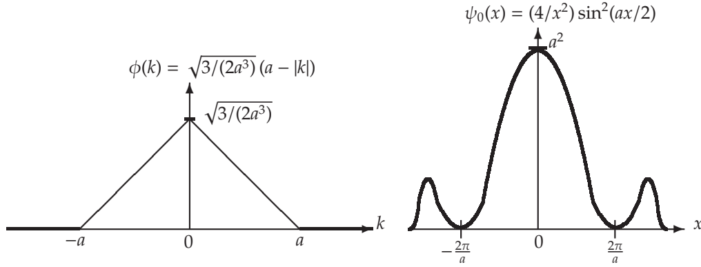
Figure 1.20: The shape of the function \phi(k) and its Fourier transform \psi_0(x) .
