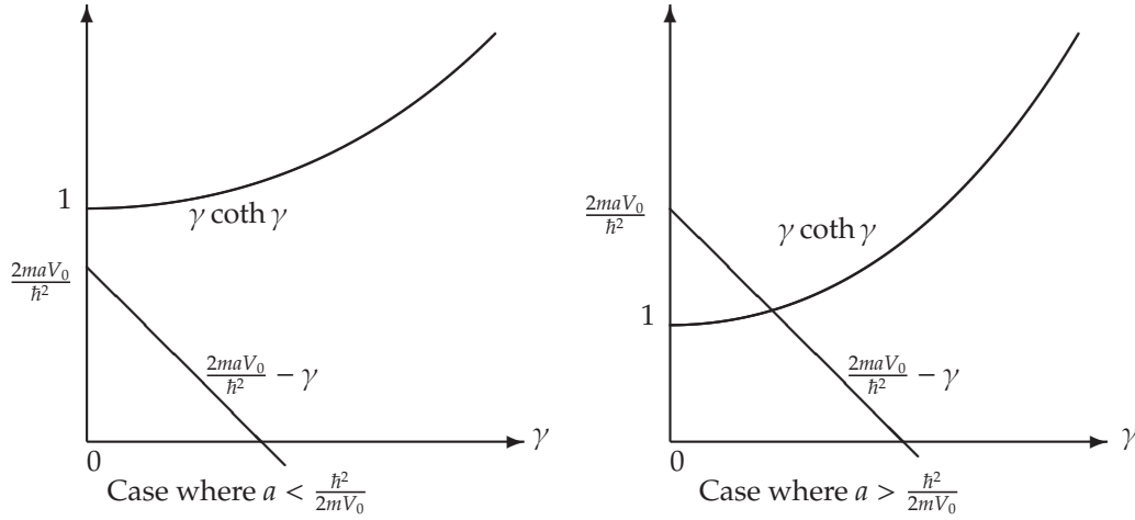
Figure 6.7: Graphical solutions of f(\gamma) = g(\gamma) , with \gamma = ka , f(\gamma) = \gamma \coth \gamma , and g(\gamma) = 2mV_0a/\hbar^2 - \gamma . If a < \hbar^2/(2mV_0) there is no bound state. If a > \hbar^2/(2mV_0) there is one bound state.
