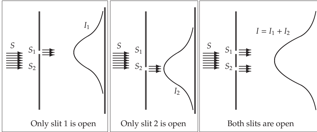
Figure 1.9: The double-slit experiment with particles : S is a source of bullets ; I_1 and I_2 are the intensities recorded on the screen, respectively, when only S_1 is open and then when only S_2 is open. When both slits are open, the total intensity is I = I_1 + I_2 .
