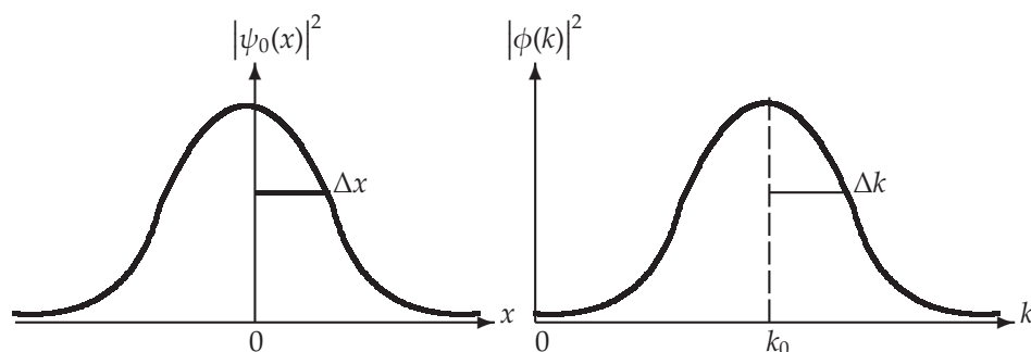
Figure 1.15: Two localized wave packets: \psi_0(x) = (2/\pi a^2)^{1/4} e^{-x^2/a^2} e^{ik_0 x} and \phi(k) = (a^2/2\pi)^{1/4} e^{-a^2(k-k_0)^2/4} ; they peak at x = 0 and k = k_0 , respectively, and vanish far away.
