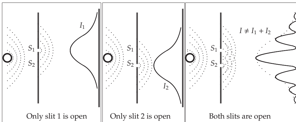
Figure 1.10: The double-slit experiment: S is a source of waves , I_1 and I_2 are the intensities recorded on the screen when only S_1 is open, and then when only S_2 is open, respectively. When both slits are open, the total intensity is no longer equal to the sum of I_1 and I_2 ; an oscillating term has to be added.
