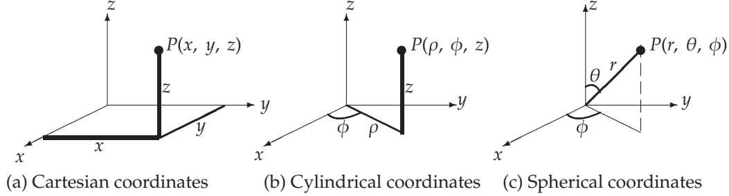
Figure D.1: Cartesian, Cylindrical, and Spherical coordinates
