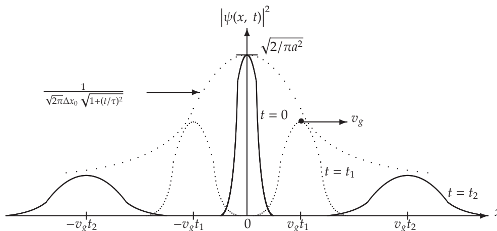
Figure 1.17: Time evolution of |\psi(x, t)|^2 : the peak of the packet, which is centered at x = v_g t , moves with the speed v_g from left to right. The height of the packet, represented here by the dotted envelope, is modulated by the function 1/(\sqrt{2\pi}\Delta x(t)) , which goes to zero at t \rightarrow \pm\infty and is equal to \sqrt{2/\pi a^2} at t = 0 . The width of the packet \Delta x(t) = \Delta x_0 \sqrt{1 + (t/\tau)^2} increases linearly with time.
