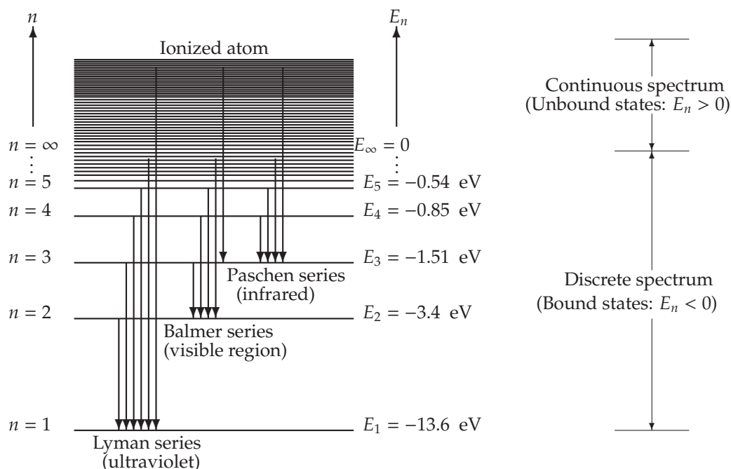
Figure 1.13: Energy levels and transitions between them for the hydrogen atom.
