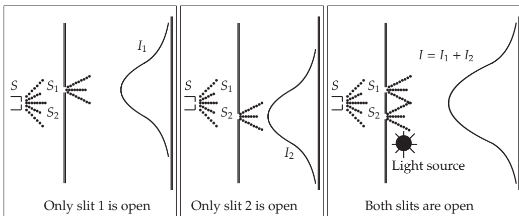
Figure 1.12: The double-slit experiment: S is a source of electrons . A light source is placed behind the wall containing S_1 and S_2 . When both slits are open, the interference pattern is destroyed and the total intensity is I = I_1 + I_2 .
