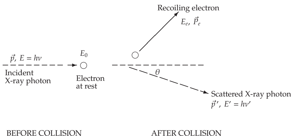
Figure 1.5: Compton scattering of an X-ray photon (of energy h\nu and momentum \vec{p} ) off a free, stationary electron. After collision, the X-ray photon is scattered at angle \theta with energy h\nu' .
