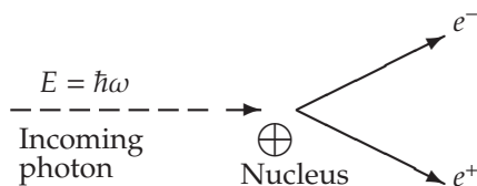
Figure 1.6: Pair production: a highly energetic photon, interacting with a nucleus, disappears and produces an electron and a positron.
