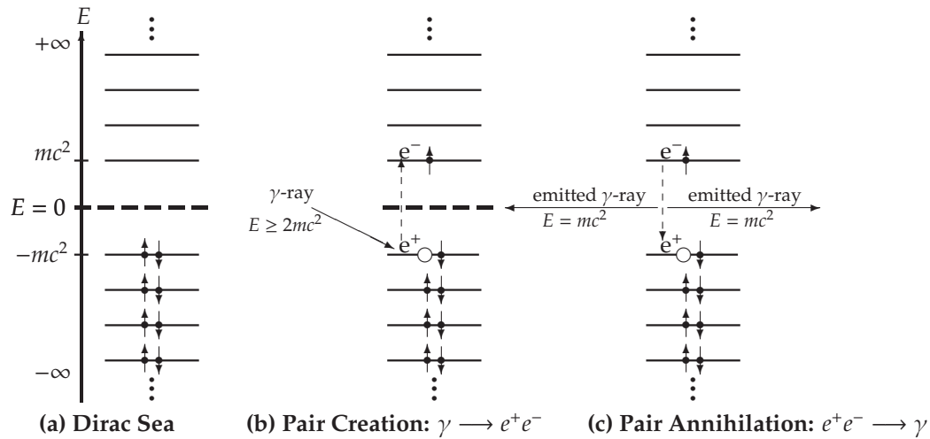
Figure 12.3: (a) Dirac Sea (vacuum): consists of an infinite continuum of negative energy states -\infty < E \leq -mc^2 that are fully occupied by electrons and the positive energy states empty. (b) Electron-Positron Pair Creation: A \gamma -ray (with a minimum energy of 2mc^2 ) is absorbed by a negative energy electron and making a transition to a positive energy state leaving behind a positron (positively charged hole). (c) Electron-Positron Pair Annihilation: A positive energy electron annihilates a positron by emitting two \gamma -rays, each with energy mc^2 , moving in opposite directions to conserve momentum.
