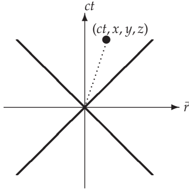
Figure E.2: Spacetime diagram where the location of an event in the Minkowski spacetime is represented by a set of four coordinates (ct, x, y, z) where \vec{r} stands for (x, y, z) .
