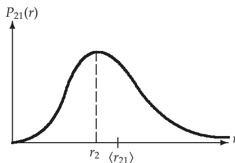
Figure 6.6: The probability density P_{21}(r) = r^4 e^{-r/a_0} / (24a_0^5) is asymmetric about its maximum r_2 = 4a_0 ; the average of r is \langle r_{21} \rangle = 5a_0 and the width of the probability density is \Delta r_{21} = \sqrt{5}a_0 .
