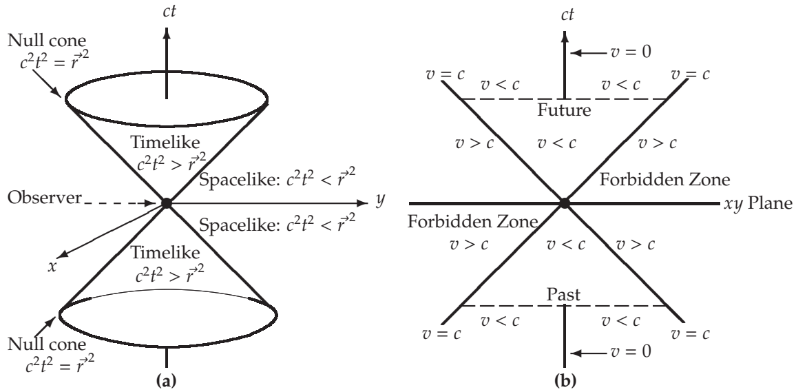
Figure E.3: (a): Conventional three-dimensional light cone diagram with 2-space xy -dimensions (the z -dimension is suppressed) and one time dimension. (b): Two-dimensional representation of the light cone diagram of an event (with speed v ).
