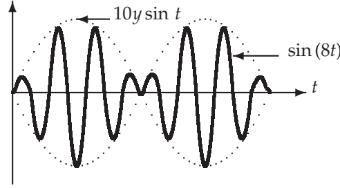
Figure 1.21: Shape of the wave packet \psi(y, t) = 10y \sin t \sin 8t . The function \sin 8t , the solid curve, is modulated by 10y \sin t , the dashed curve.
