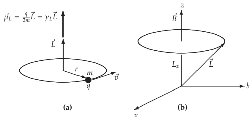
Figure 5.4: (a): Orbital magnetic dipole moment of a positive charge q orbiting with speed v along a circle of radius r is \vec{\mu}_L = \gamma_L \vec{L} where \gamma_L = q/(2m) . (b): When an external magnetic field is applied, the orbital magnetic moment precesses about it.
