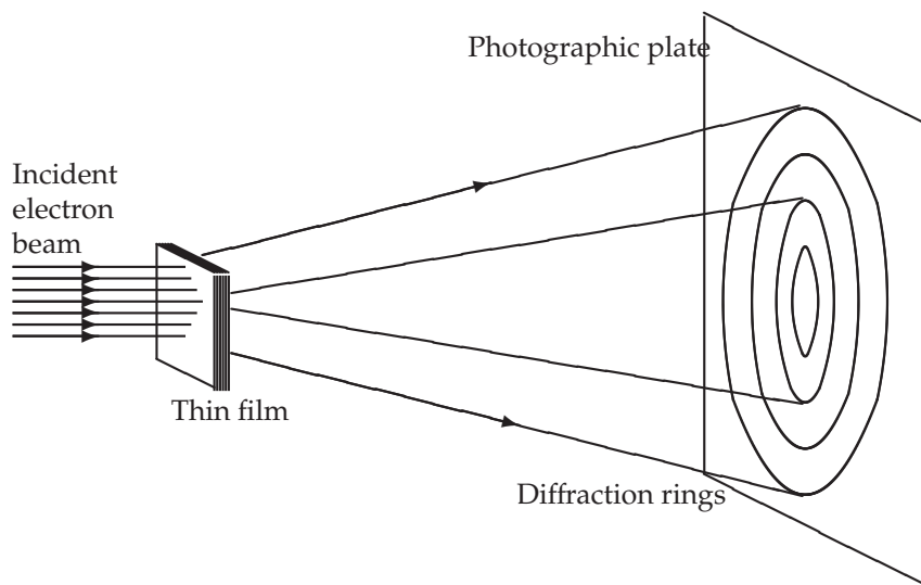
Figure 1.8: Thomson experiment: diffraction of electrons through a thin film of polycrystalline material yields fringes that usually result from light diffraction.
