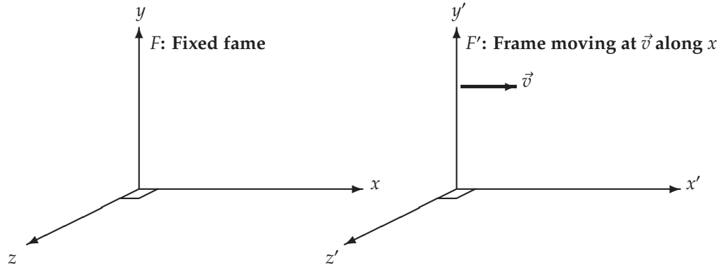
Figure E.1: Inertial frames F and F' : F is fixed while F' is moving at constant velocity \vec{v} along the positive x -axis
