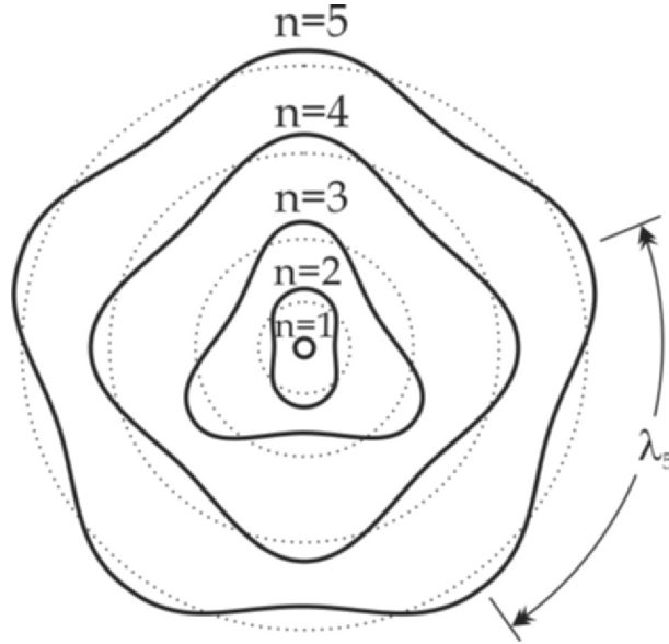
Figure 1.14: Illustration of the five lowest orbits of the electron in a hydrogen atom where the electron is represented by a wave as per de Broglie's matter-wave hypothesis.
