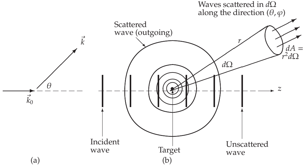
Figure 11.3: (a) Angle between the incident and scattered wave vectors \vec{k}_0 and \vec{k} . (b) Incident and scattered waves: the incident wave is a plane wave, \phi_{inc}(\vec{r}) = A e^{i\vec{k}_0 \cdot \vec{r}} , and the scattered wave, \phi_{sc}(\vec{r}) = A f(\theta, \varphi) \frac{e^{i\vec{k} \cdot \vec{r}}}{r} , is an outgoing wave.
