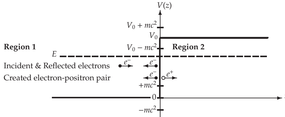
Figure 12.5: Scattering of electrons of energy E from a step potential V_0 where E < V_0 - mc^2 .
