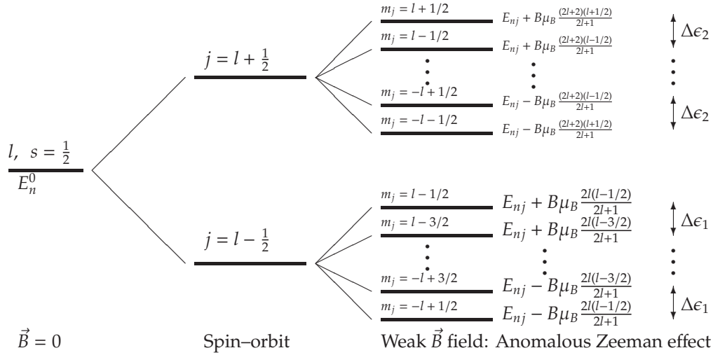
Figure 9.3: Splittings of a level l due to the spin-orbit interaction and to a weak external magnetic field, with E_{nj} = E_n^0 + E_{SO}^{(1)} . All the lower sublevels are equally spaced, \Delta\epsilon_1 = B\mu_B(2l)/(2l+1) , and so are the upper sublevels, \Delta\epsilon_2 = B\mu_B(2l+2)/(2l+1) , with \mu_B = e\hbar/(2m_e) .
