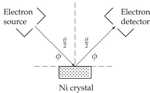
Figure 1.7: Davisson–Germer experiment: electrons strike the crystal’s surface at an angle \phi ; the detector, symmetrically located from the electron source, measures the number of electrons scattered at an angle \theta , where \theta is the angle between the incident and scattered electron beams.
