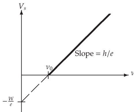
Figure 1.4: Stopping potential V_s as a function of the radiation's frequency \nu .
