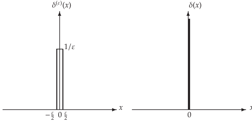
Figure A.1: The delta function \delta(x) as defined by \delta(x) = \lim_{\epsilon \rightarrow 0} \delta^{(\epsilon)}(x) .
