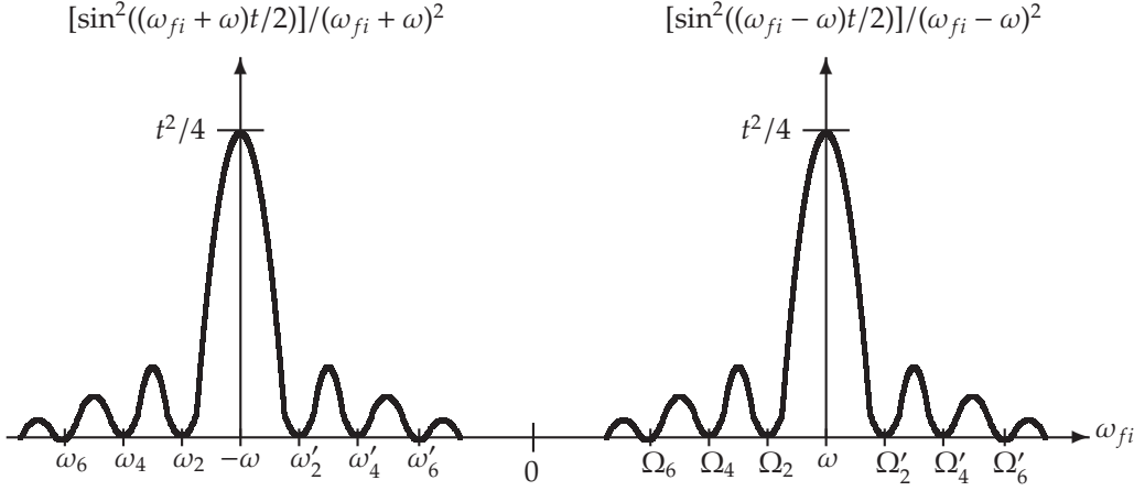
Figure 10.2: Plot of [\sin^2((\omega_{fi} \pm \omega)t/2)]/(\omega_{fi} \pm \omega)^2 versus \omega_{fi} for a fixed value of t , where \omega_n = -\omega - n\pi/t , \omega'_n = -\omega + n\pi/t , \Omega_n = \omega - n\pi/t , and \Omega'_n = \omega + n\pi/t .
