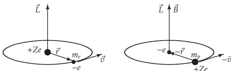
Figure 9.1: (Left) An electron moving in a circular orbit as seen by the nucleus. (Right) The same motion as seen by the electron within its rest frame; the electron sees the nucleus moving in a circular orbit around it.
