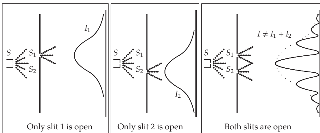
Figure 1.11: The double-slit experiment: S is a source of electrons , I_1 and I_2 are the intensities recorded on the screen when only S_1 is open, and then when only S_2 is open, respectively. When both slits are open, the total intensity is equal to the sum of I_1 , I_2 and an oscillating term.
