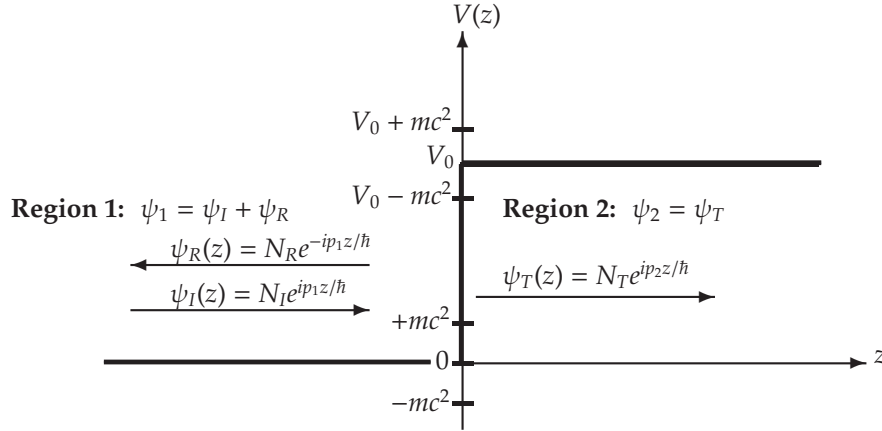
Figure 12.1: Scattering of a free relativistic, spinless particle from a Step potential V_0 ; the propagation directions of the incident, reflected, and transmitted waves corresponding to the energy range E > V_0 + mc^2 are shown in the figure.
