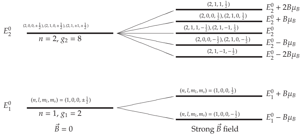
Figure 9.2: Splittings of the energy levels n = 1 and n = 2 of a hydrogen atom when placed in a strong external magnetic field; \mu_B = e\hbar/(2m_e) .
