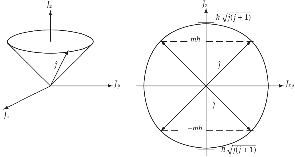
Figure 5.1: Geometrical representation of the angular momentum \hat{\mathbf{J}} : the vector \hat{\mathbf{J}} rotates along the surface of a cone about its axis; the cone's height is equal to m\hbar , the projection of \hat{\mathbf{J}} on the cone's axis. The tip of \hat{\mathbf{J}} lies, within the J_z J_{xy} plane, on a circle of radius \hbar \sqrt{j(j+1)} .
