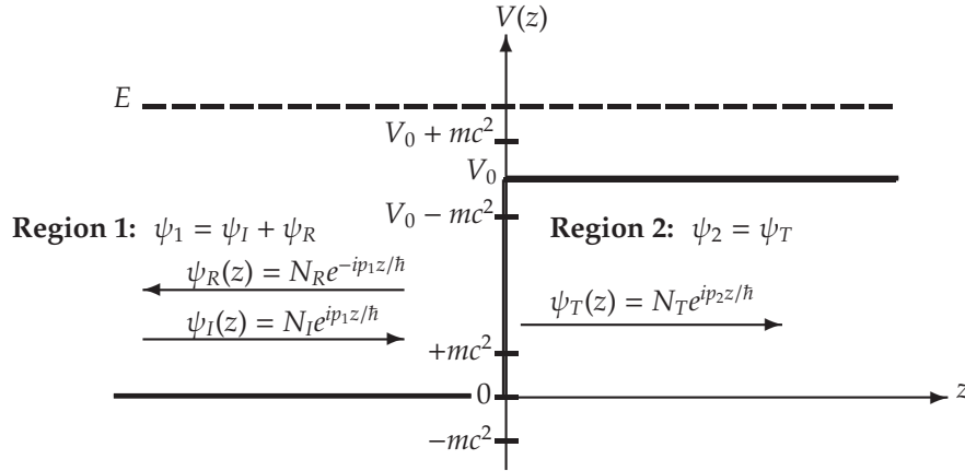
Figure 12.7: The incident, reflected, and transmitted waves pertaining to a free electron moving to the right with an energy E > V_0 + mc^2 and striking a step potential V_0 .
