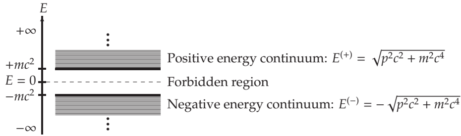
Figure 12.2: Energy spectrum of a free Dirac particle: It consists of two energy continua (allowed regions) that are separated by a forbidden region of width 2mc^2 ; the positive energy band, E^{(+)} > mc^2 , corresponds to particles and the negative energy band, E^{(-)} < -mc^2 , to antiparticles.
