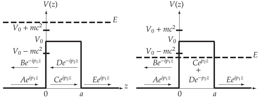
Figure 12.8: Potential barrier and propagation directions of the incident, reflected, and transmitted waves when E > V_0 + mc^2 and E < V_0 - mc^2 .
