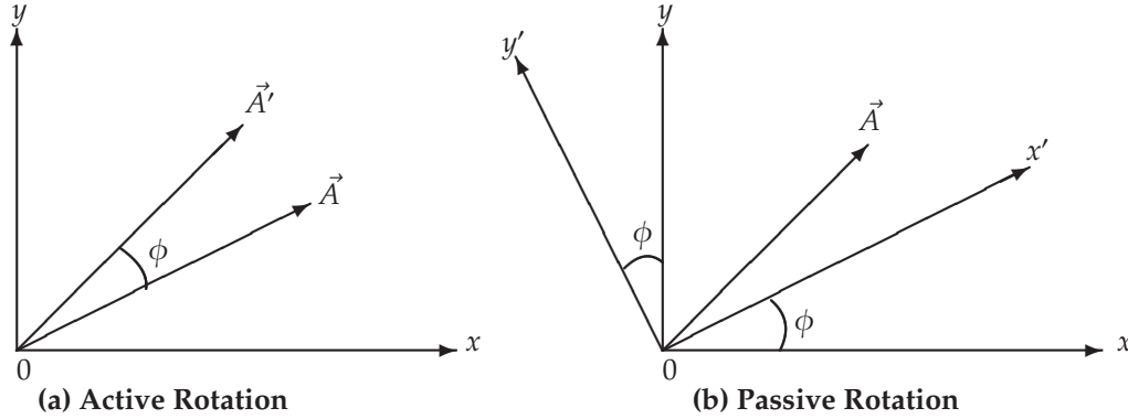
Figure 7.1: (a) Active rotation: Keeping the xy -coordinate system fixed, we rotate the vector \vec{A} = A_x\hat{i} + A_y\hat{j} counterclockwise through an angle \phi about the z -axis into the new vector \vec{A}' = A'_x\hat{i} + A'_y\hat{j} ; (b) Passive Rotation: Keeping the vector \vec{A} intact, we rotate the xy -system counterclockwise through an angle \phi about the z -axis into the new x'y' -system; vector \vec{A} is expressed by \vec{A} = A_x\hat{i} + A_y\hat{j} and \vec{A} = A'_x\hat{i}' + A'_y\hat{j}' in the xy and x'y' systems, respectively.
