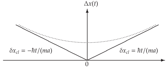
Figure 1.18: Time evolutions of the packet's width \Delta x(t) = \Delta x_0 \sqrt{1 + (\delta x_{cl}(t)/\Delta x_0)^2} (dotted curve) and of the classical dispersion \delta x_{cl}(t) = \pm \hbar t/(ma) (solid lines). For large values of |t| , \Delta x(t) approaches \delta x_{cl}(t) and at t = 0 , \Delta x(0) = a/2 .
