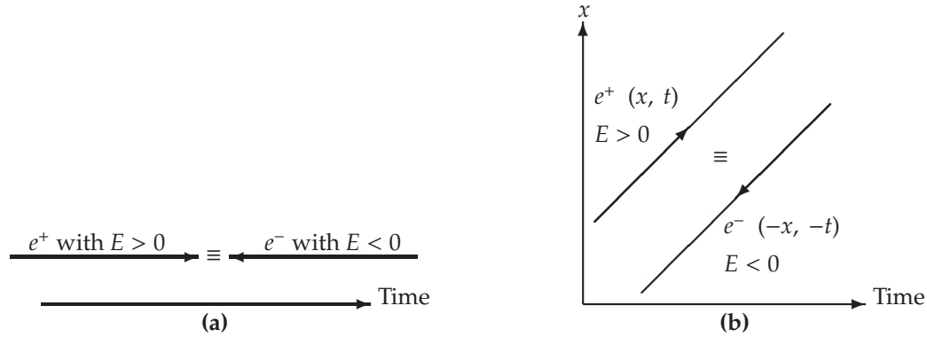
Figure 12.4: Pictorial view of the Feynman-Stückelberg interpretation of the negative energy solutions: (a) : using only the time variable, (b) : using space and time: The solution of a negative energy particle (electron) traveling backwards in space and time (-x, -t) is equivalent to that of a positive energy antiparticle (positron) traveling forwards in space and time (x, t) .
