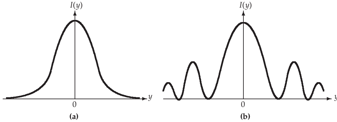
Figure 1.19: Shape of the total intensity generated in a double slit experiment when both slits are open and (a) a light source is used to observe the electrons' motion, I(y) = 2/\pi(1 + y^2) , and no interference is registered; (b) no light source is used , I(y) = 4/[\pi(1 + y^2)] \cos^2(\pi y/2) , and an interference pattern occurs.
