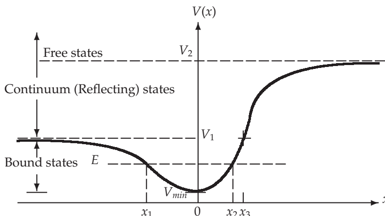
Figure 4.1: Shape of a general potential displaying discrete (bound) and continuous (reflecting and free) states.
